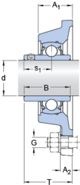
FY 1.3/16 TF/VA201 Bearing 2D drawings and 3D CAD models
