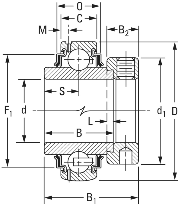
G1013KRRB Bearing 2D drawings and 3D CAD models
